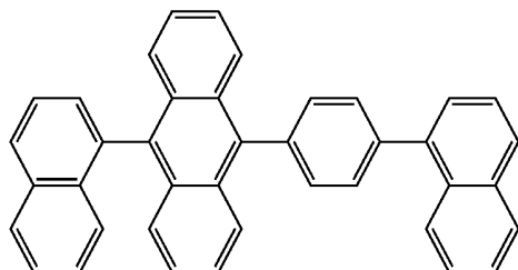
[Chemical Formula 8]
