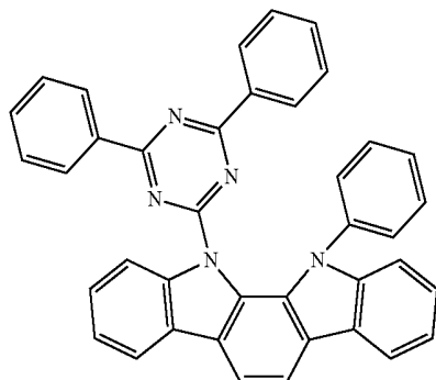
[Chemical Formula 1-1]
