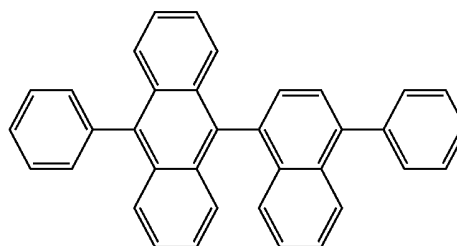
[Chemical Formula 2-1]
