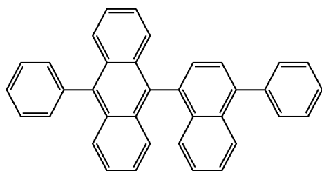
[Chemical Formula 2-1 to Chemical Formula 2-8]
