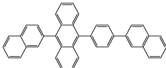
[Chemical Formula 8]
